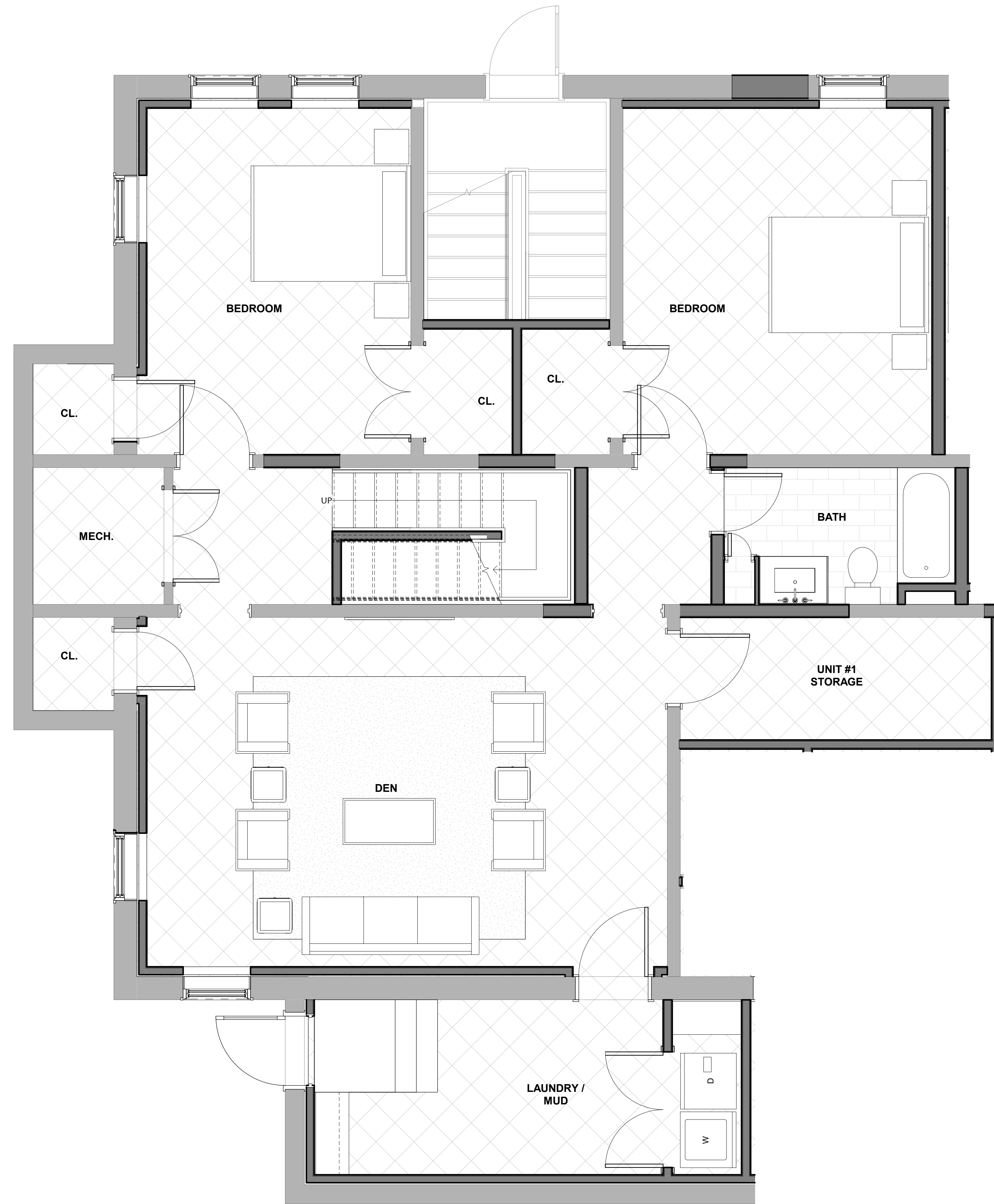
① PROPOSED LOWER LEVEL PLAN 3/8" = 1'-0"
